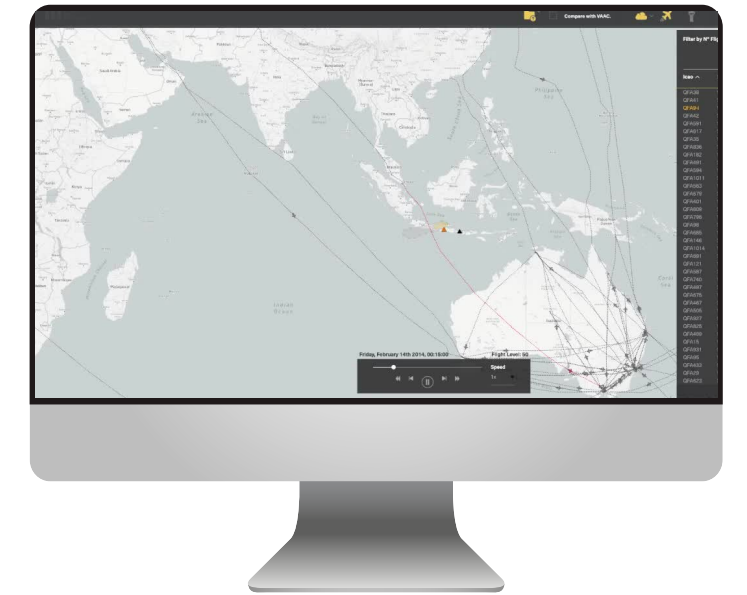
Volcanoes
