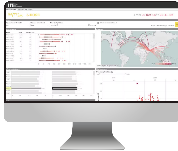
Atmospheric aerosols
